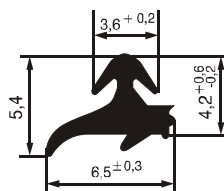
№ 07330402 G: 19 g/m Hardness acc. Shore °A - 75 ±5
