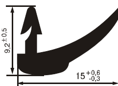
№ 07320202 G: 53 g/m Hardness acc. Shore °A - 75 ±5
