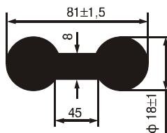
№ 07300102 G: 1250 g/m Hardness acc. Shore °A > 90
