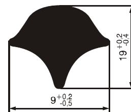
№ 07320102 G: 55 g/m Hardness acc. Shore °A - 75 ±5
