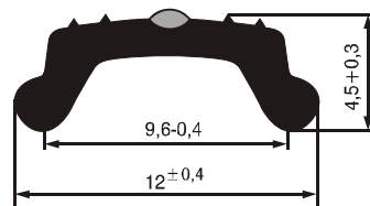
№ 07321002 G: 30 g/m Hardness acc. Shore °A - 75 ±5
