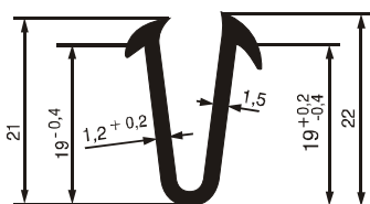
№ 07320602 G: 68 g/m Hardness acc. Shore °A - 75 ±5
