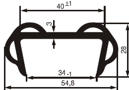
№ 07330202 G: 450 g/m Hardness acc. Shore °A - 65 ±5
