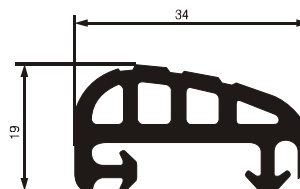
№ 07321002 G: 30 g/m Hardness acc. Shore °A - 75 ±5
