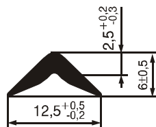
№ 07320002 G: 35 g/m Hardness acc. Shore °A - 75 ±5
