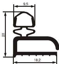
№ 07400002 G: 100 g/m Hardness acc. Shore °A - 77 ±3
