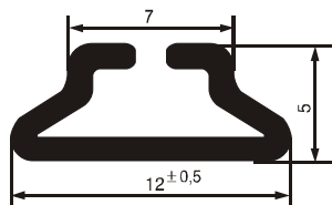
№ 07320802 G: 36 g/m Hardness acc. Shore °A - 75 ±5
