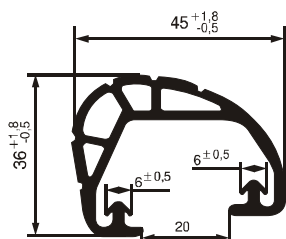
№ 07330002 G: 480 g/m Hardness acc. Shore °A - 65 ±5
