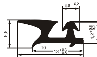
№ 07320502 G: 39 g/m Hardness acc. Shore °A - 75 ±5
