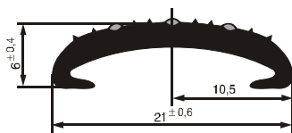
№ 07321102 G: 56 g/m Hardness acc. Shore °A - 75 ±5
