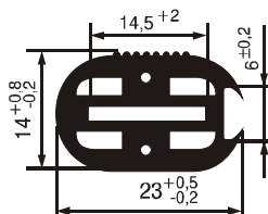
№ 07310002 G: 235 g/m Hardness acc. Shore °A - 85 ±5
