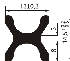
№ 07320702 G: 100 g/m Hardness acc. Shore °A - 75 ±5
