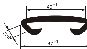
№ 07340002 G: 400 g/m Hardness acc. Shore °A - 85 ±5
