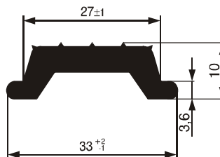
№ 07310102 G: 195 g/m Hardness acc. Shore °A 85±5
