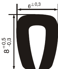
№ 07321202 G: 39 g/m Hardness acc. Shore °A - 75 ±5
