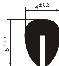
№ 07321302 G: 14 g/m Hardness acc. Shore °A - 75 ±5
