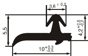
№ 07320402 G: 25 g/m Hardness acc. Shore °A - 75 ±5
